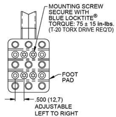
FOOT PAD DETAIL
